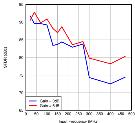
Figure 7-53. SFDR vs Input Frequency
