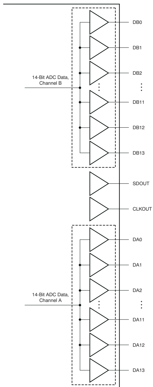
Figure 8-24. CMOS Outputs
