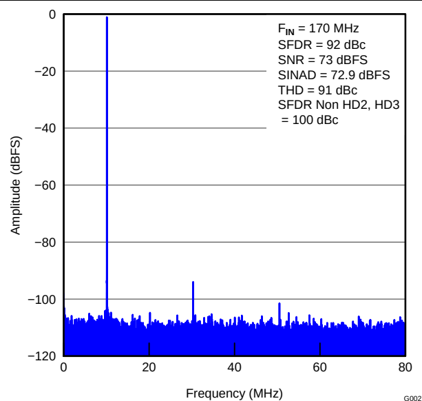
Figure 88. FFT for 170-MHz Input Signal
