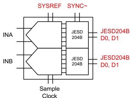
Figure 46. JESD204B Interface
