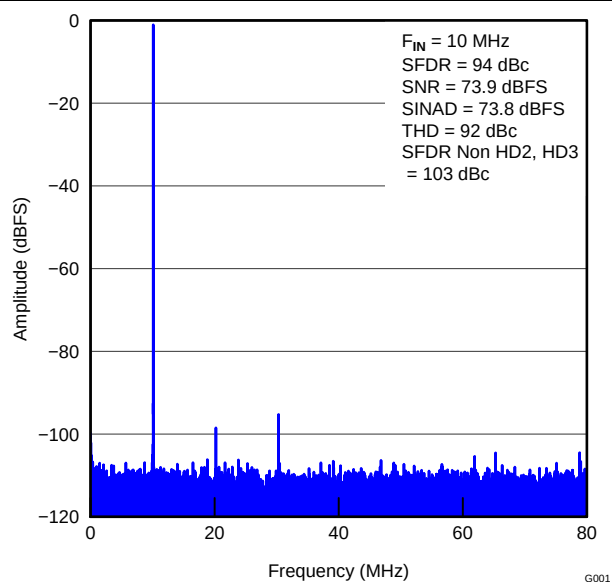
Figure 87. FFT for 10-MHz Input Signal
