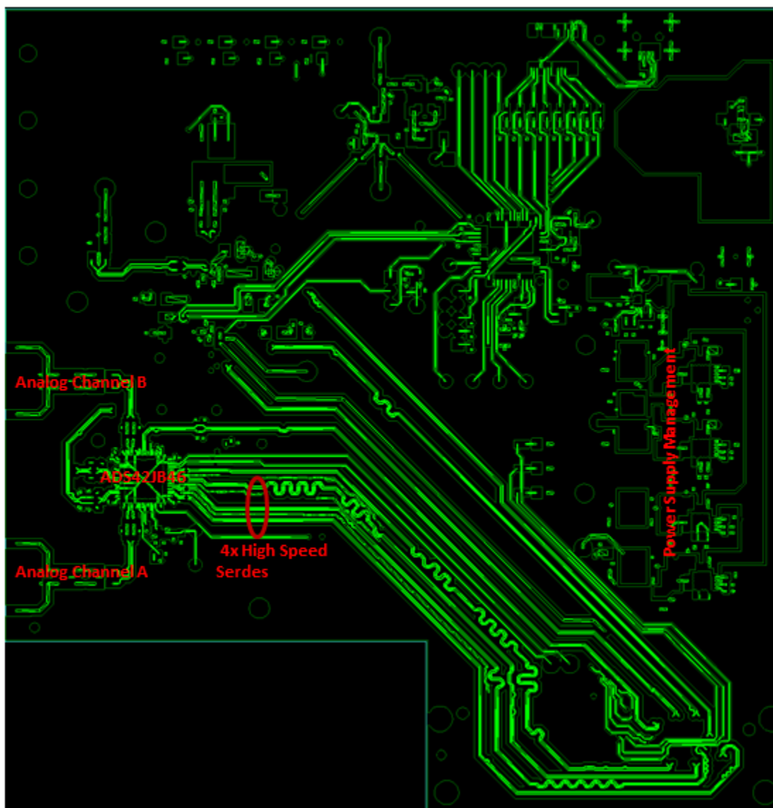
Figure 91. Layout Recommendation
