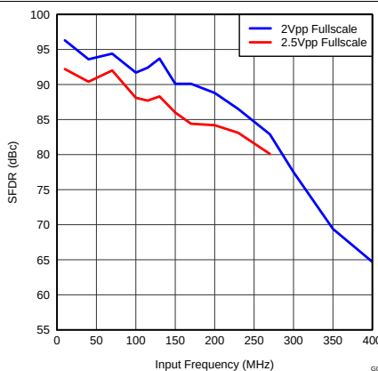
Figure 18. Spurious-Free Dynamic Range vs Input Frequency
