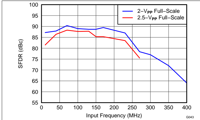
Figure 43. SFDR vs Input Frequency
