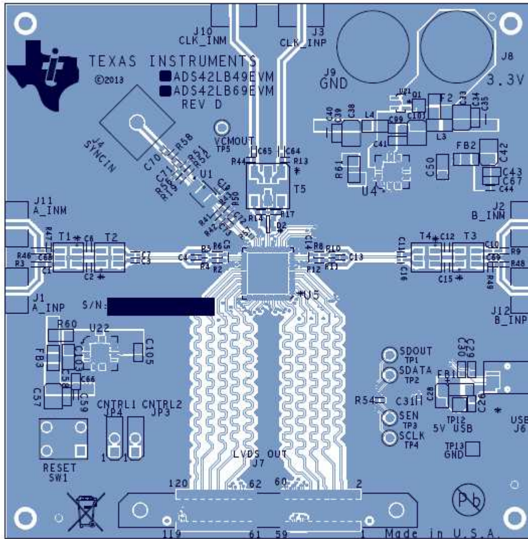
Figure 127. Example Layout
