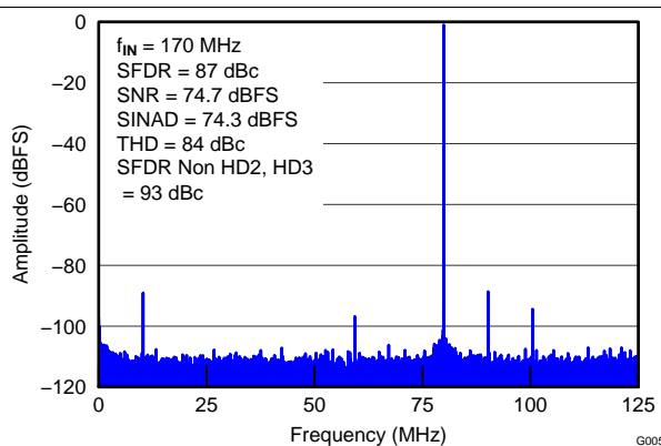
Figure 5. FFT for 170-MHz Input Signal (2.5- V_{\text{PP}} Full-Scale)
