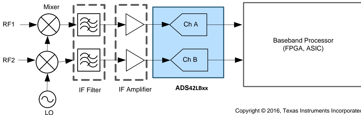
Figure 109. The ADS42LBx9 in a Dual-Channel Superheterodyne Receiver
