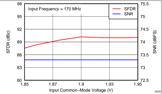
Figure 20. Performance vs Input Common-Mode Voltage (170 MHz)
