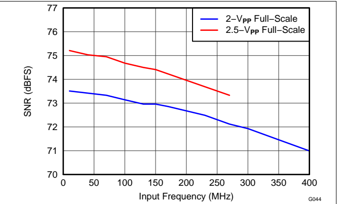
Figure 44. SNR vs Input Frequency
