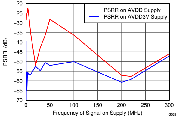
Input Frequency = 10 MHz 50-mV PP Signal Superimposed on Supply
