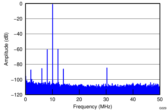
Amplitude ( f_{IN} ) = -1 dBFS Amplitude ( f_{PSRR} ) = -87 dBFS f_{IN} = 10 MHz Amplitude ( f_{IN} + f_{PSRR} ) = -60.6 dBFS f_{PSRR} = 2 MHz, 50 mV PP Amplitude ( f_{IN} - f_{PSRR} ) = -60 dBFS
