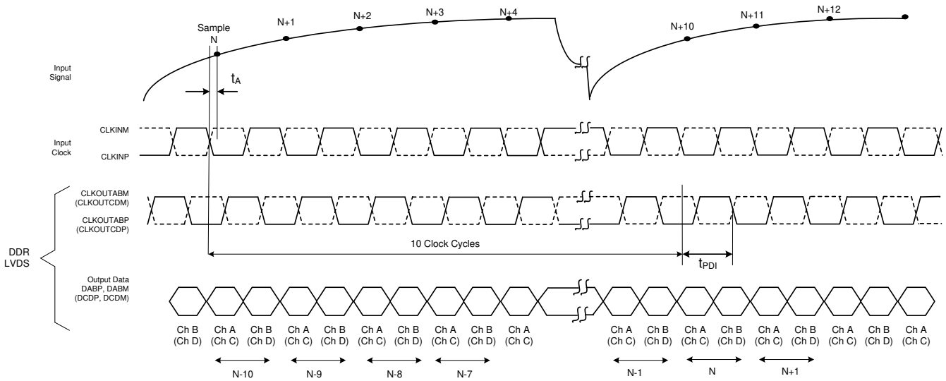
Figure 7-2. Latency Timing
