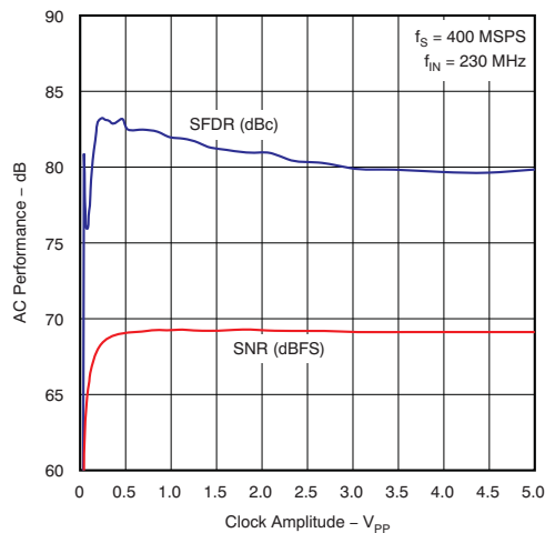
Figure 37. AC Performance vs Clock Level
