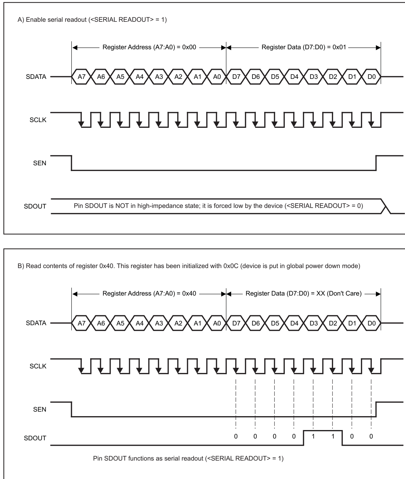
Figure 10. Serial Readout
