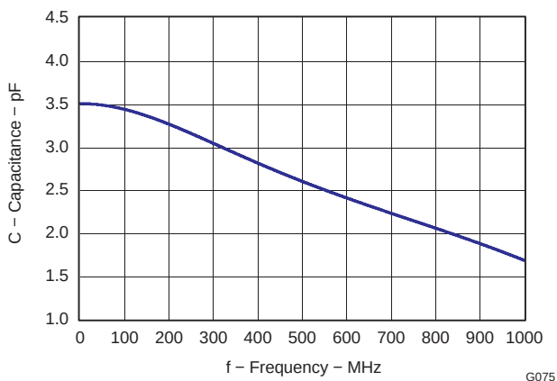
Figure 101. ADC Analog Input Capacitance (Cin) Across Frequency
