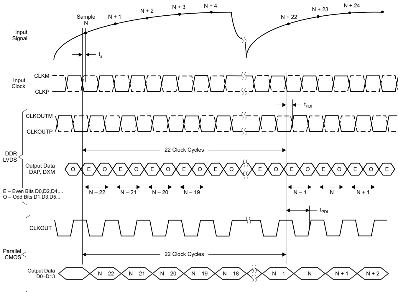
Figure 5. Latency Diagram
