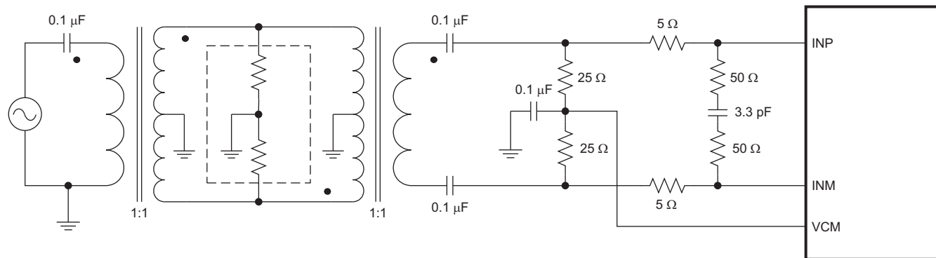
Figure 103. Drive Circuit With High Bandwidth (for high input frequencies)
