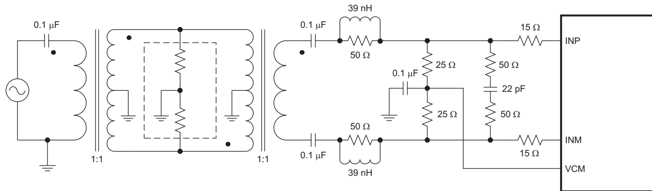
Figure 102. Drive Circuit With Low Bandwidth (for low input frequencies)
