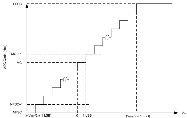
Figure 44. Ideal Transfer Characteristics for Pseudo-Differential Configuration
