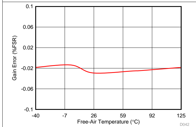
Figure 36. Gain Error in High Precision Mode with Temperature
