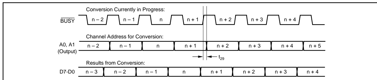
FIGURE 7. Channel Addressing in Continuous Conversion Mode (CONTC HIGH, CS and R/C LOW).
