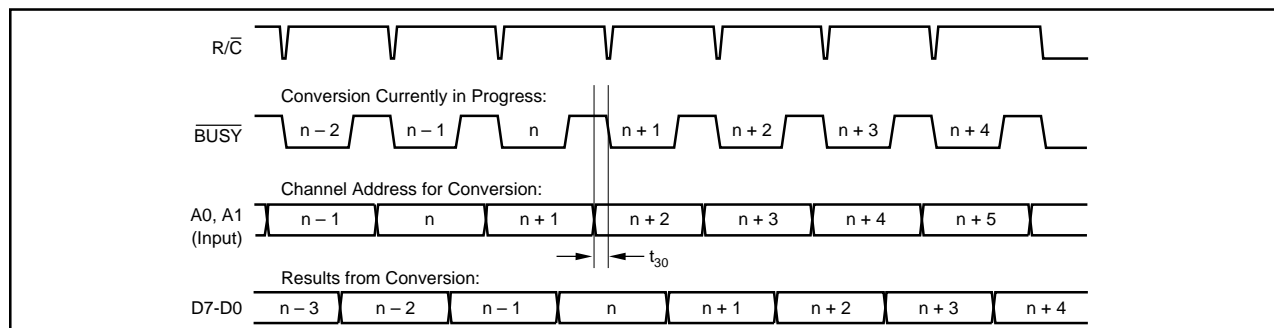
FIGURE 8. Channel Addressing in Normal Conversion Mode (CONTC and CS LOW).
