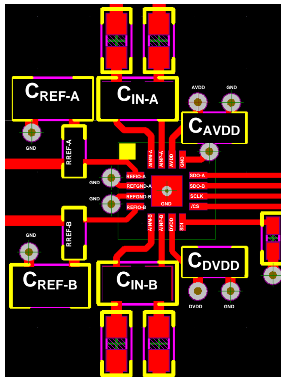
Figure 117. Recommended Layout
