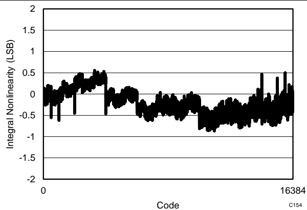
Figure 45. Typical INL
