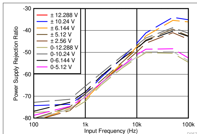
Figure 9-1. PSRR Without a Decoupling Capacitor
