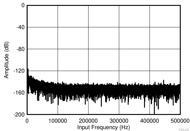
Figure 6-33. Typical FFT Plot (All Ranges) for the ADS8691
