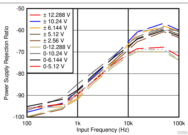
Figure 9-2. PSRR With a Decoupling Capacitor
