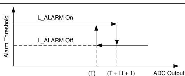
Figure 7-18. Low ALARM Hysteresis
