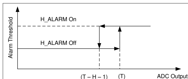
Figure 7-17. High ALARM Hysteresis
