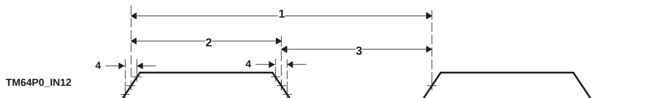
Figure 6-49. Timer Timing
