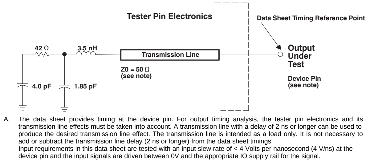
Figure 6-1. Test Load Circuit for AC Timing Measurements
