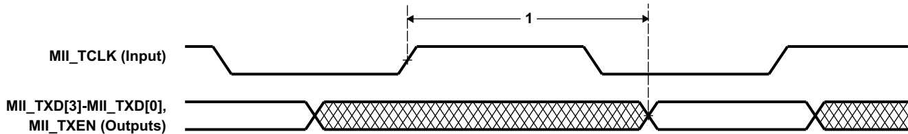
Figure 6-45. EMAC Transmit Interface Timing
