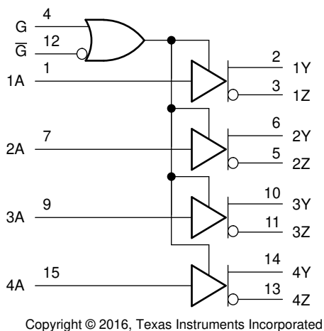
Figure 7-1. Logic Diagram
