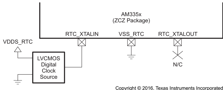
Figure 6-16. OSC1 (ZCZ Package) LVC MOS Circuit Schematic
