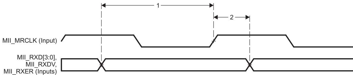
Figure 7-111. PRU-ICSS MII_RXD[3:0], MII_RXDV, and MII_RXER Timing
