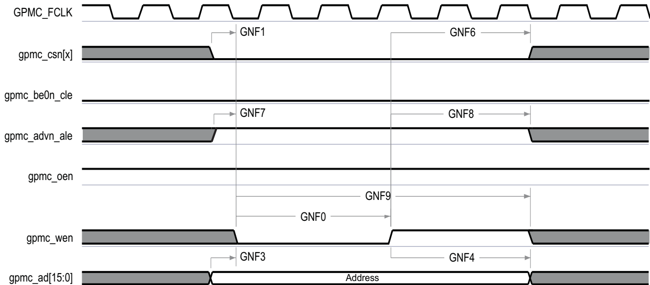
Figure 7-29. GPMC and NAND Flash—Address Latch Cycle
