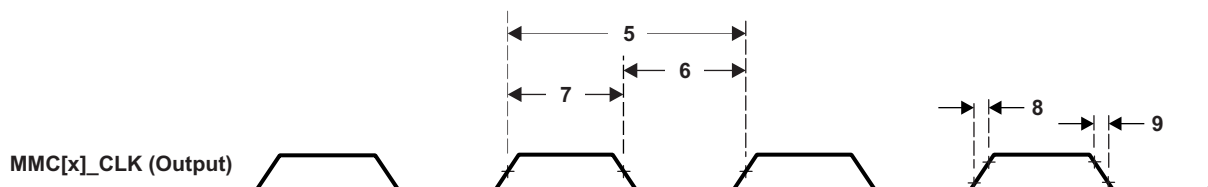
Figure 5-141. MMC[x]_CLK Timing
