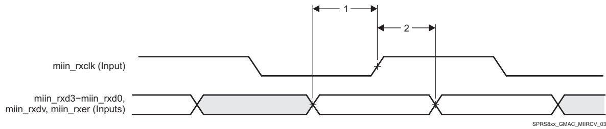
Figure 7-53. GMAC Receive Interface Timing MII operation
