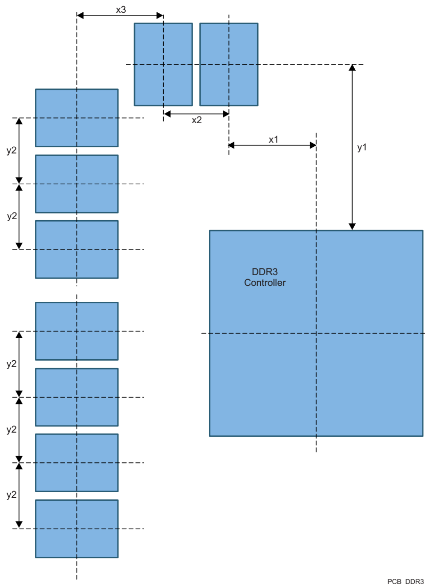
Figure 8-4. Placement Specifications
