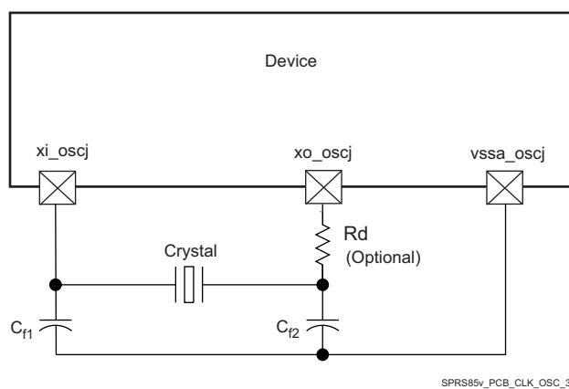
Figure 8-33. Grounding Scheme for High-Frequency Clock
