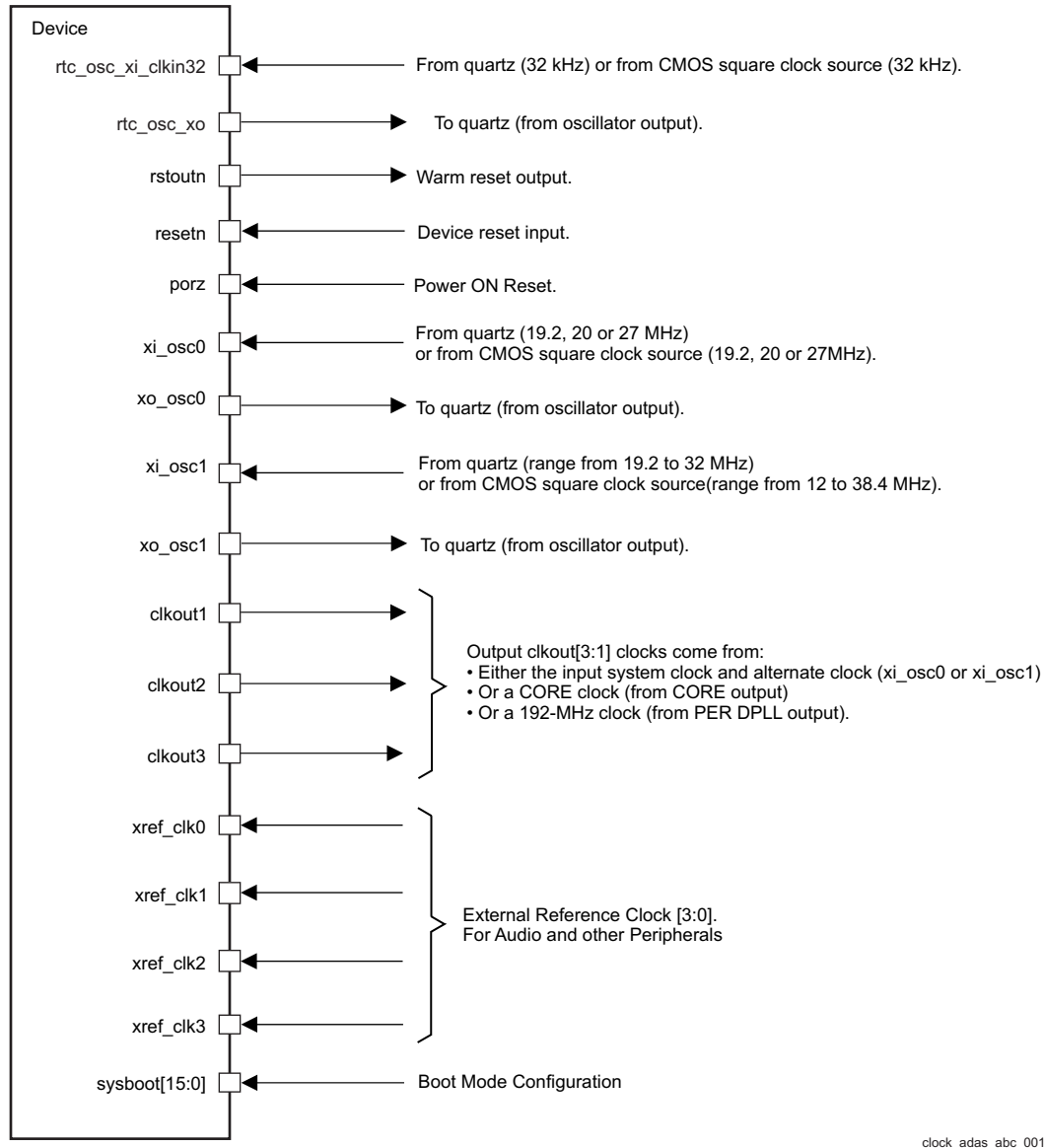
Figure 6-1. Clock Interface
