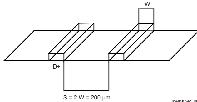
Figure 8-29. Ground Guard Illustration
