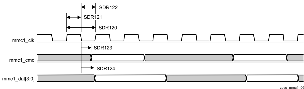
Figure 7-65. MMC/SD/SDIO in - High Speed SDR12 - Transmitter Mode
