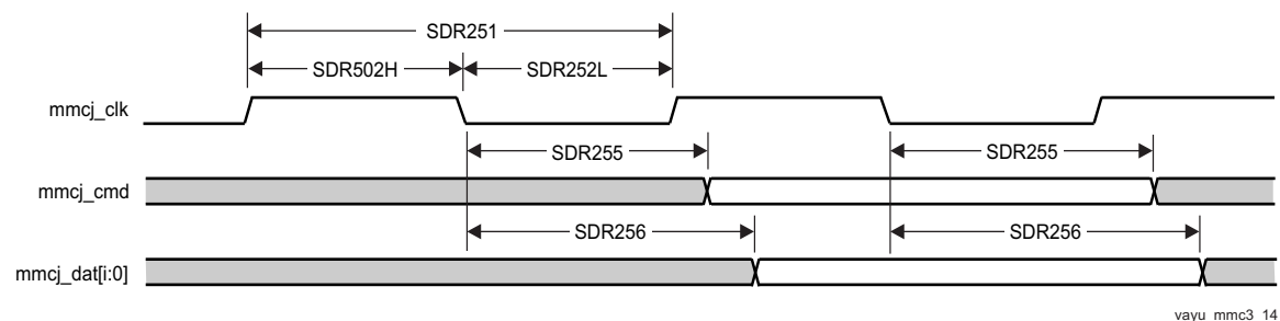
Figure 7-88. MMC/SD/SDIOj in - SDR25 - Transmitter Mode
