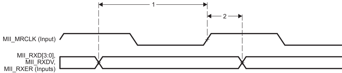
Figure 7-106. PRU-ICSS MII_RXD[3:0], MII_RXDV, and MII_RXER Timing
