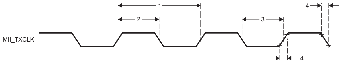
Figure 7-105. PRU-ICSS MII[x]_TXCLK Timing
