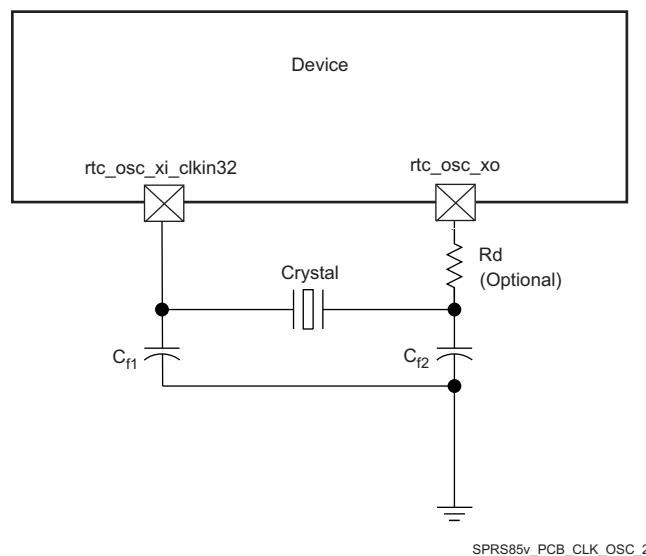
Figure 8-32. Grounding Scheme for Low-Frequency Clock
