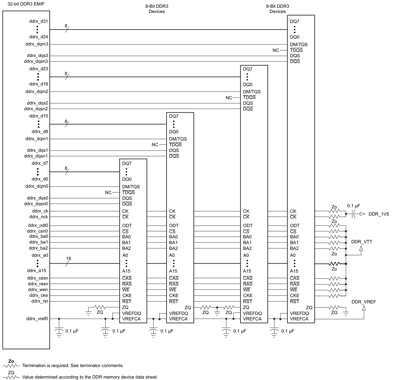
Figure 8-3. 32-Bit, One-Bank DDR3 Interface Schematic Using Four 8-Bit DDR3 Devices
