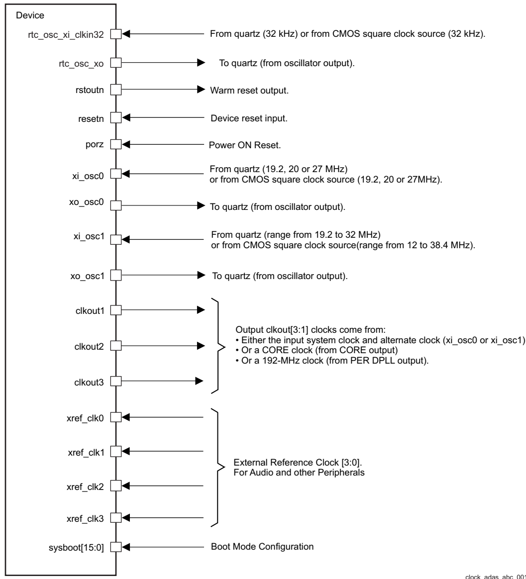
Figure 6-1. Clock Interface
