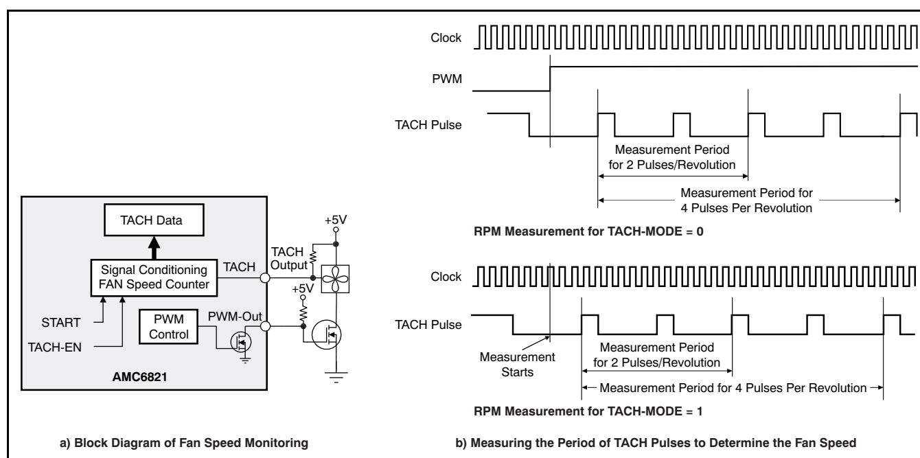
Figure 17. Fan Speed Measurement
