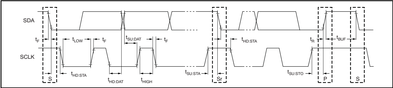
Figure 1. Timing Specification
