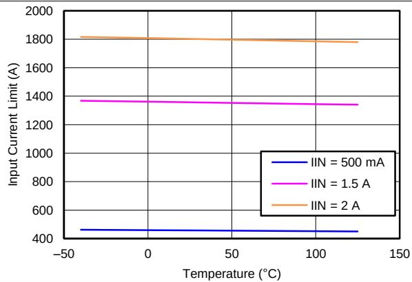
Figure 8. Input Current Limit vs Temperature
