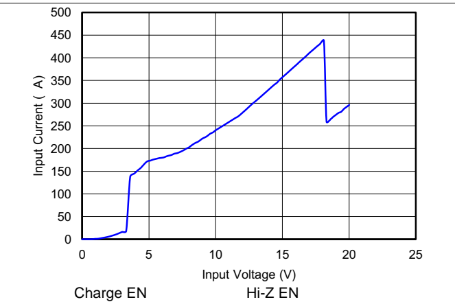
Figure 10. Input IQ with Charge Enable and Hi-Z
