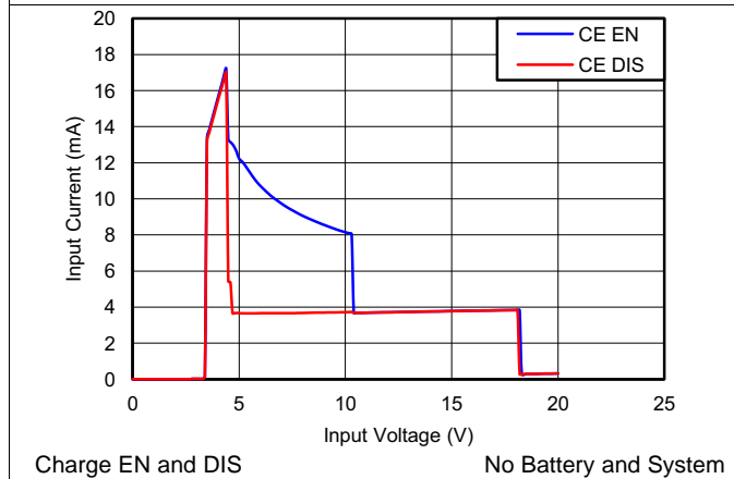
Figure 9. Input IQ With Charge DIS and EN
