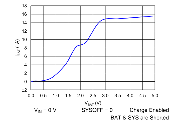
Figure 7. BAT IQ, SYSOFF = 0
