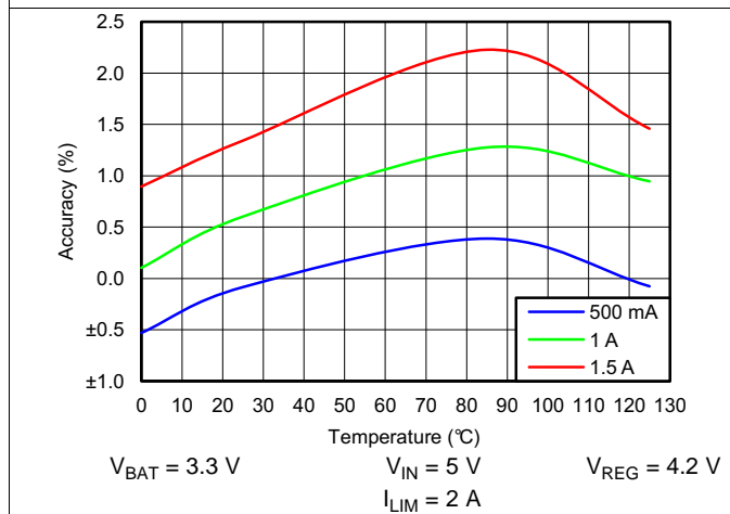
Figure 11. I_{CHG} Accuracy with Internal Settings, V_{BAT} = 3.3 V
