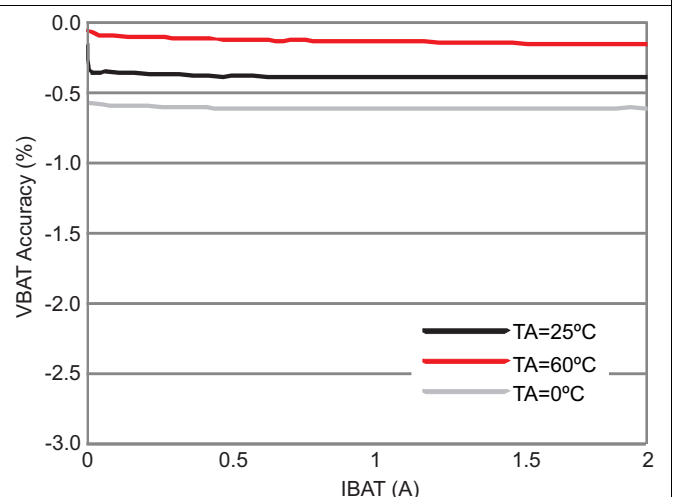
Figure 4. VBAT Accuracy vs IBAT – 4.2-V Setting
