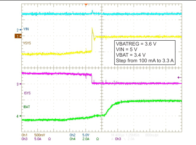
Figure 36. VSYS Transient With Supplement Mode
