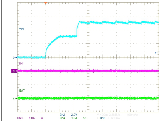
Figure 37. Boost Start-up No Load
