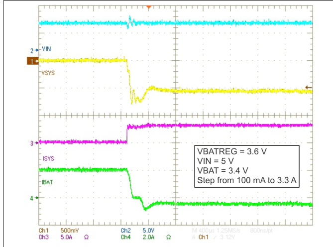
Figure 35. VSYS Transient With Supplement Mode
