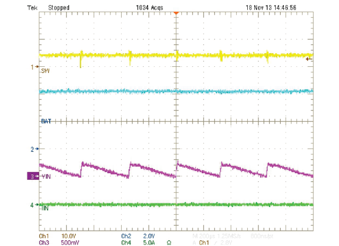
Figure 38. Boost Burst Mode During Light Load
