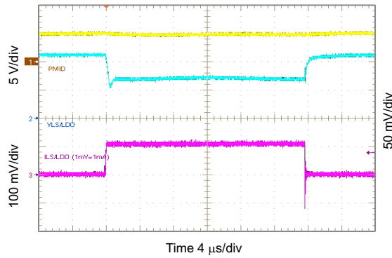
Figure 89. 1.2 V_{LSLDO} Load Transient, 0 to 100 mA
