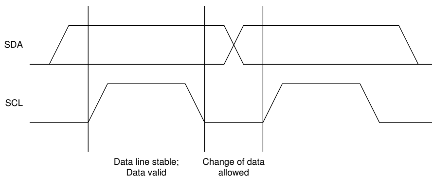
Figure 9-12. Bit Transfer on the I 2 C Bus
