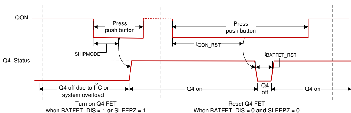
Figure 9-10. \overline{QON} Timing
