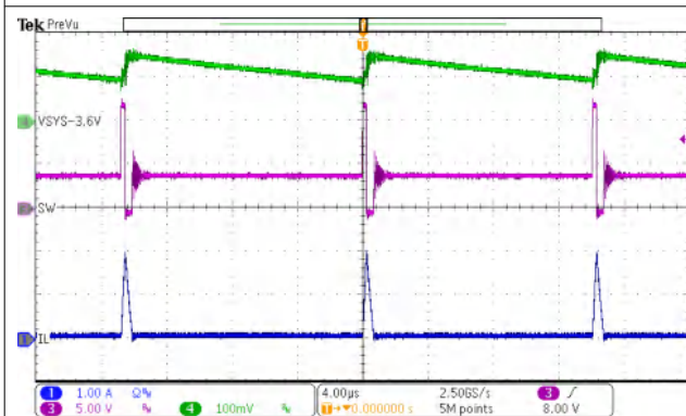
V_{VBUS} = 12\text{ V} Charge Disabled I_{SYS} = 50\text{ mA} Figure 10-6. PFM Switching in Buck Mode
