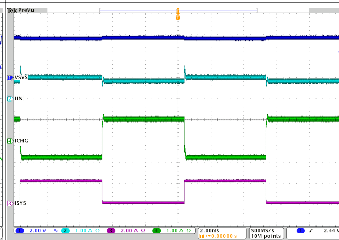
Figure 10-11. OTG Switching
