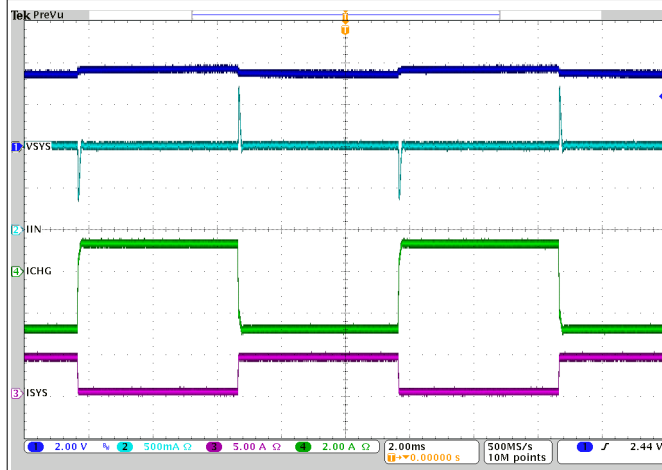
Figure 10-14. System Load Transient
