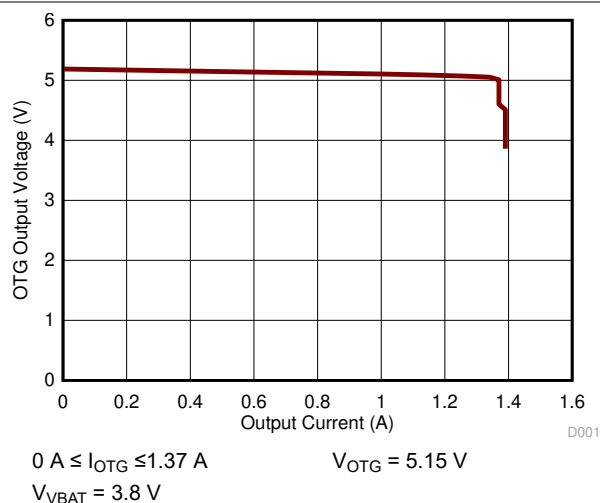
Figure 8-3. OTG Output Voltage vs. Output Current
