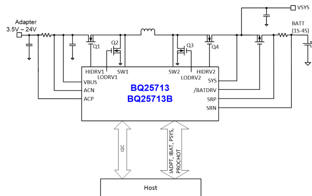
Application Diagram
