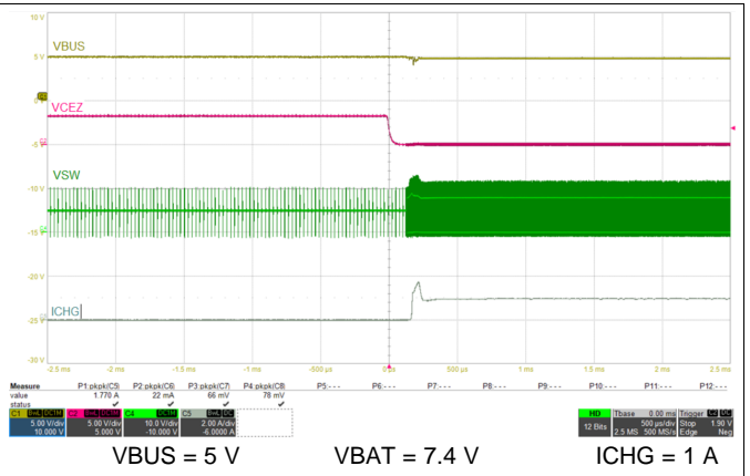
Figure 22. Charge Enable
