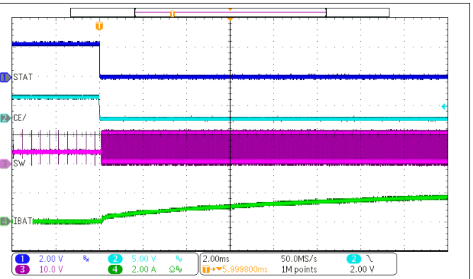
Figure 48. Charge Enable
