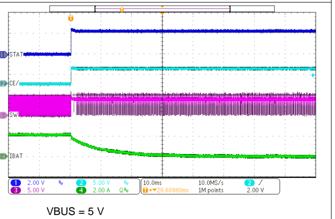
Figure 44. Charge Disable
