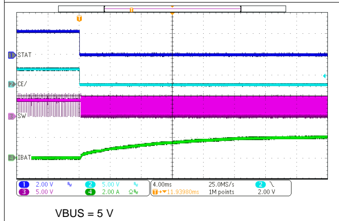
Figure 43. Charge Enable
