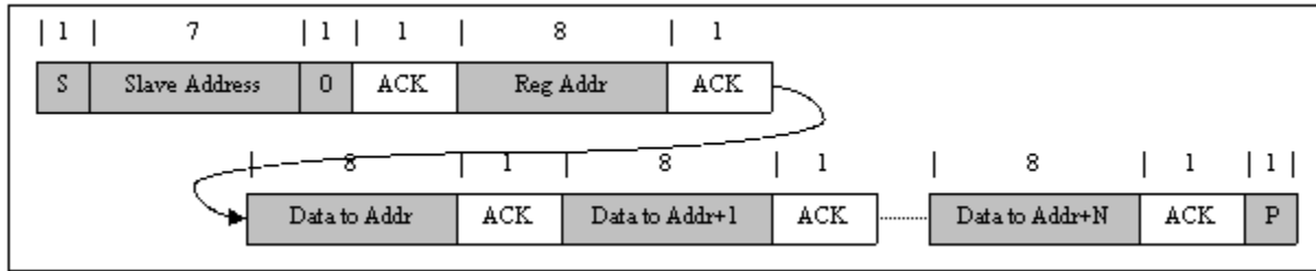
Figure 17. Multi-Write
