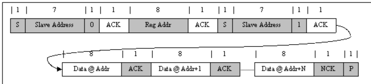
Figure 18. Multi-Read
