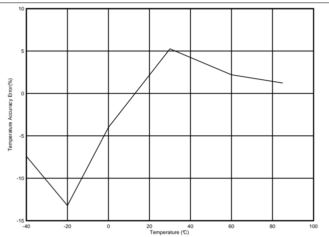
Figure 8. Temperature Accuracy
