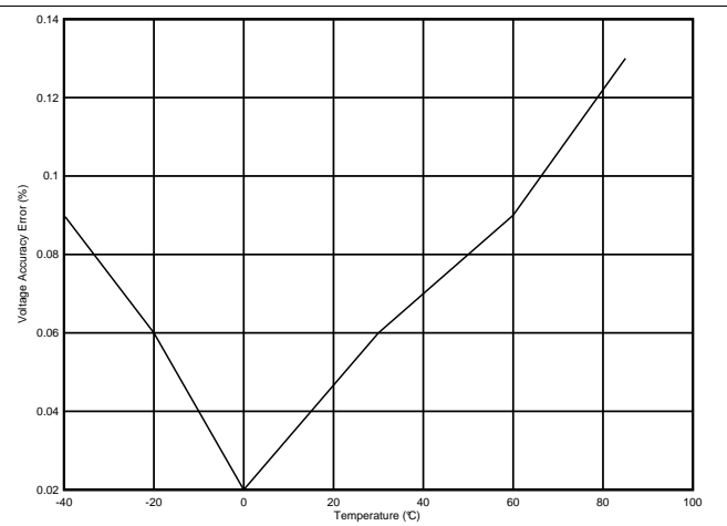
Figure 11. Temperature Accuracy
