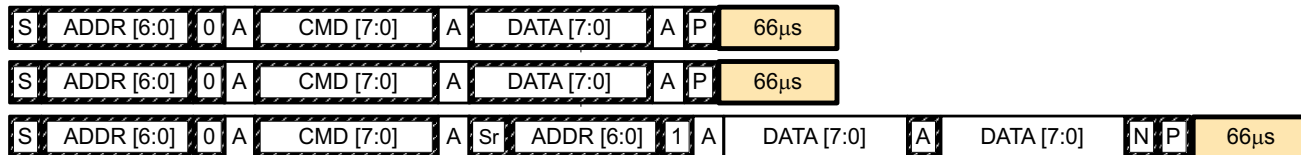
Waiting time inserted between two 1-byte write packets for a subcommand and reading results (required for 100 kHz < f_{SCL} \leq 400 kHz)
