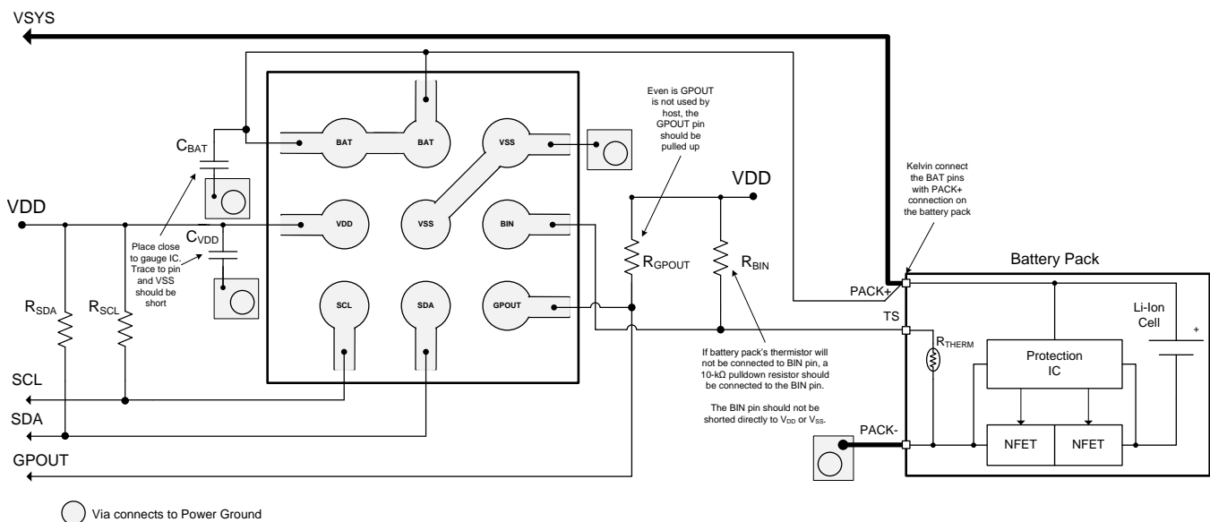
Figure 13. Layout Example
