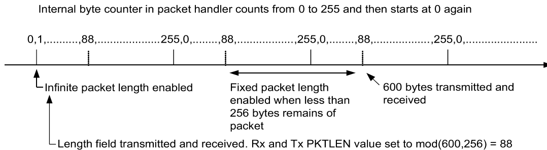
Figure 20: Packet Length > 255
