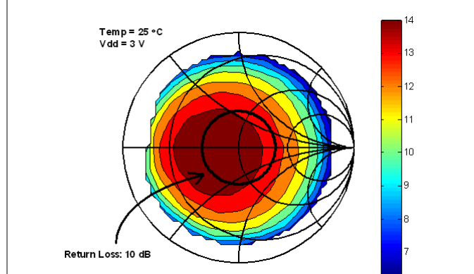
Figure 6-6. Output Power vs Load Impedance (+14-dBm Setting)
