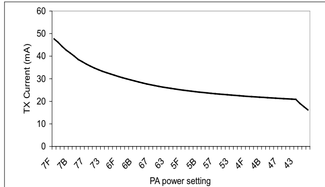
Figure 6-1. TX Current at 868 MHz vs PA Power Setting
