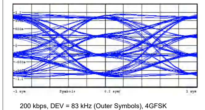
Figure 6-5. Eye Diagram
