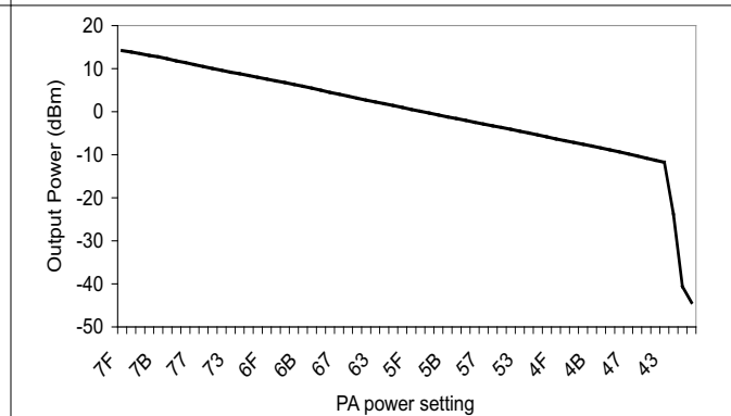
Figure 6-4. Output Power at 868 MHz vs PA Power Setting
