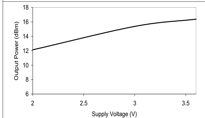
Figure 6-3. Output Power vs Voltage Max Setting, 170 MHz
