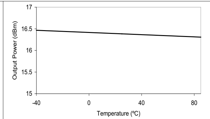
Figure 6-2. Output Power vs Temperature Max Setting, 170 MHz, 3.6 V
