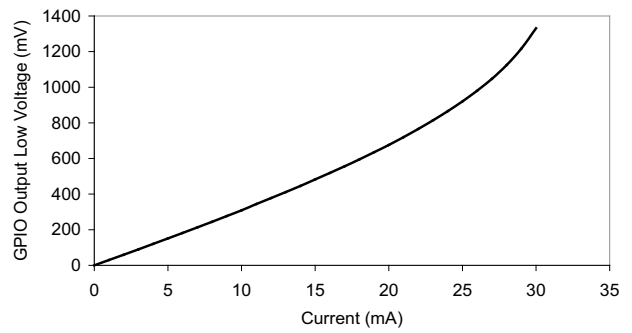
Figure 6-10. GPIO Output Low Voltage vs Current Being Sunk
