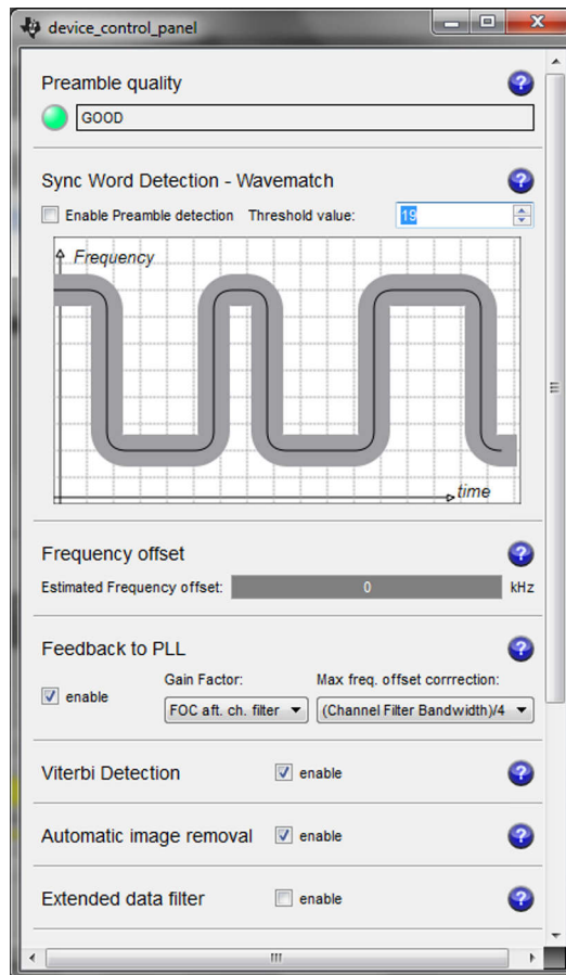
Figure 7-2. Receiver Configurator in SmartRF® Studio
