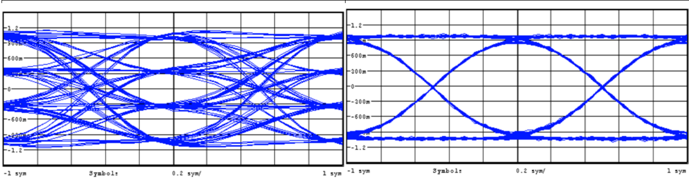
1.2 kbps 2-FSK, DEV = 4 kHz Figure 4-14. Eye Diagram
