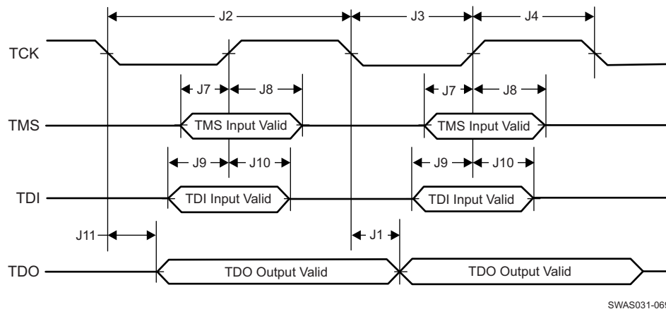
Figure 4-19. JTAG Timing
