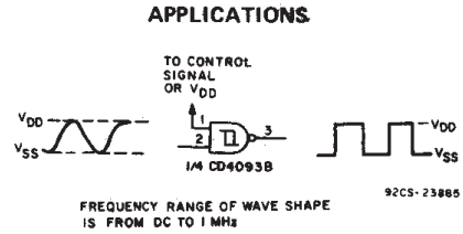
Fig. 16 – Wave shaper.
