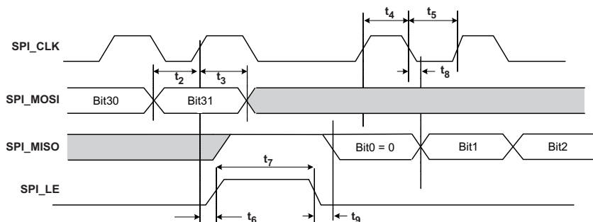
Figure 2. Timing Diagram for SPI Read Command
