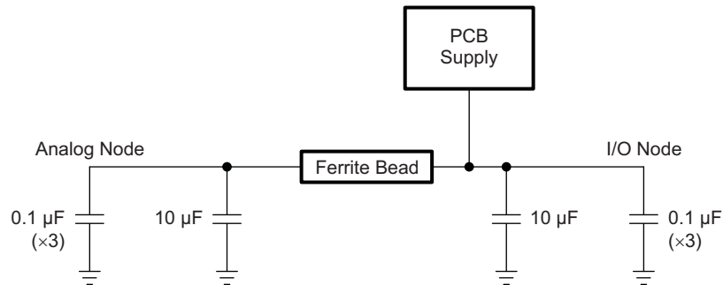
Figure 20. CDCM9102 Power Supply Decoupling – Power Pin Bypass Concept
