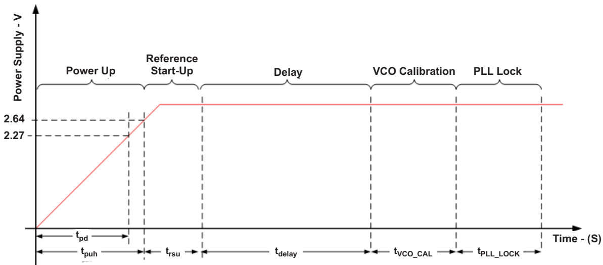
Figure 10. CDCM9102 Start-Up Time Dependencies
