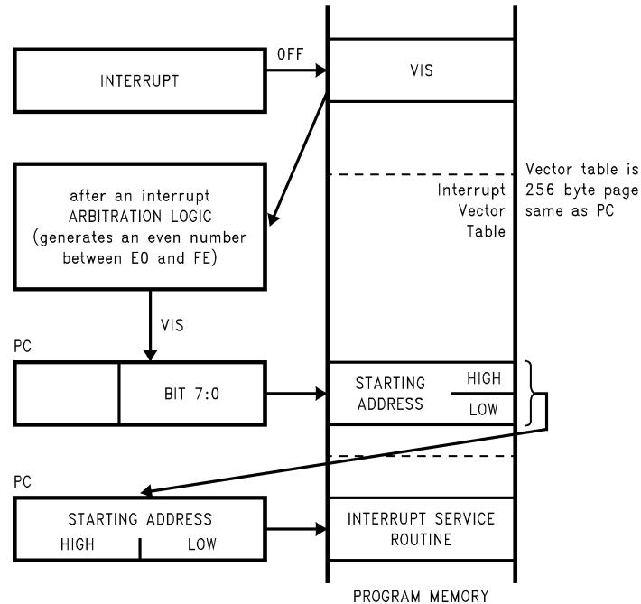
FIGURE 22. VIS Operation
