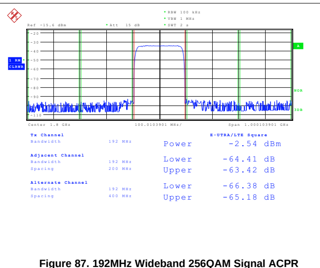
Figure 87. 192MHz Wideband 256QAM Signal ACPR
