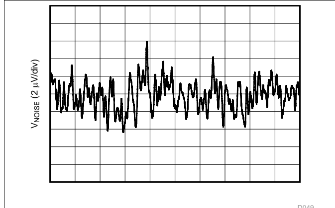
Gain = 1. External Reference = 2.5 V. DAC code at midscale
