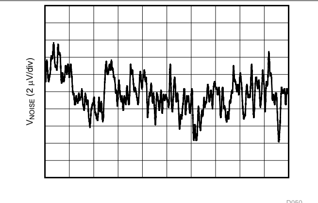
Gain = 1. DAC code at midscale
