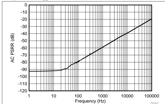
Gain = 1. V_{DD} = 5\text{ V} + 200\text{ mV}_{PP} (Sinusoid). DAC code at fullscale
