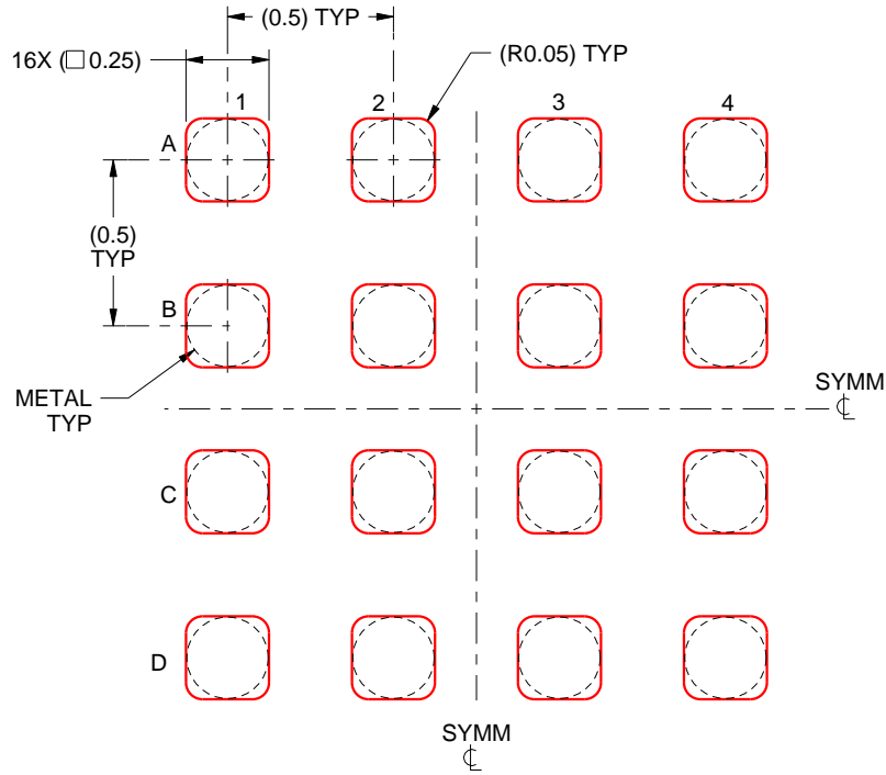
SOLDER PASTE EXAMPLE BASED ON 0.1 mm THICK STENCIL SCALE:40X
