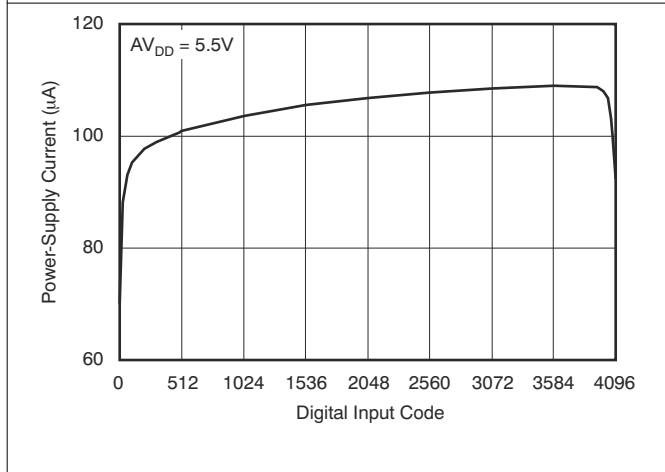
Figure 7-16. Power-Supply Current vs Digital Input Code
