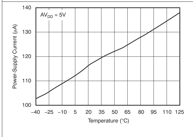
Figure 7-18. Power-Supply Current vs Temperature
