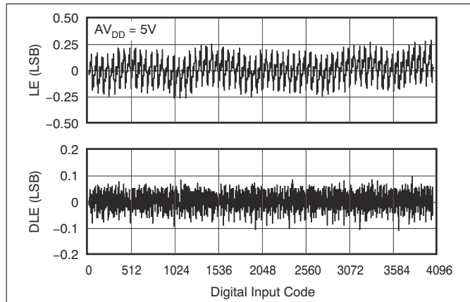
Figure 7-2. DAC7311 12-Bit Linearity Error and Differential Linearity Error vs Code ( -40^\circ\text{C} )
