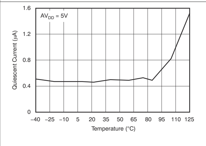
Figure 7-19. Power-Down Current vs Temperature
