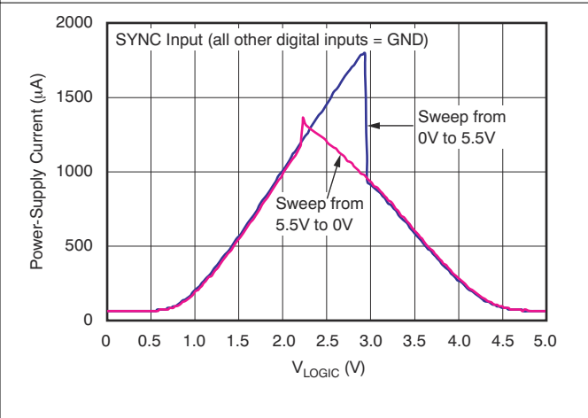
Figure 7-17. Power-Supply Current vs Logic Input Voltage
