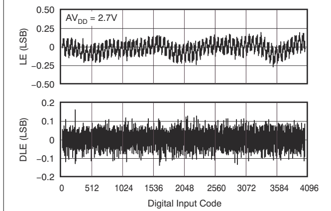
Figure 7-46. DAC7311 12-Bit Linearity Error and Differential Linearity Error vs Code ( 25^\circ\text{C} )
