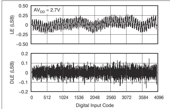
Figure 7-44. DAC7311 12-Bit Linearity Error and Differential Linearity Error vs Code ( -40^\circ\text{C} )
