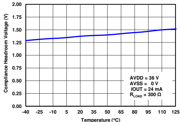
Figure 7-70. Compliance Headroom Voltage (1) vs Temperature
