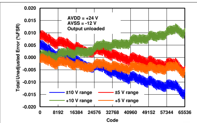
Figure 7-16. VOUT TUE vs Code
