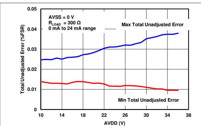
Figure 7-52. IOUT TUE vs Supply (External R_{SET} )
