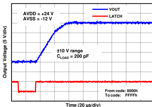
Figure 7-34. BP10V Rising
