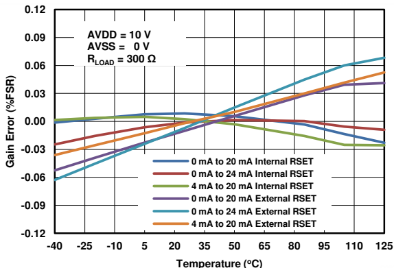
Figure 7-69. IOUT Gain Error vs Temperature
