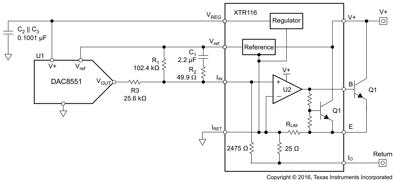
Figure 33. Loop-Powered Transmitter
