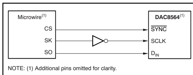
Figure 102. DAC8564 to Microwire Interface
