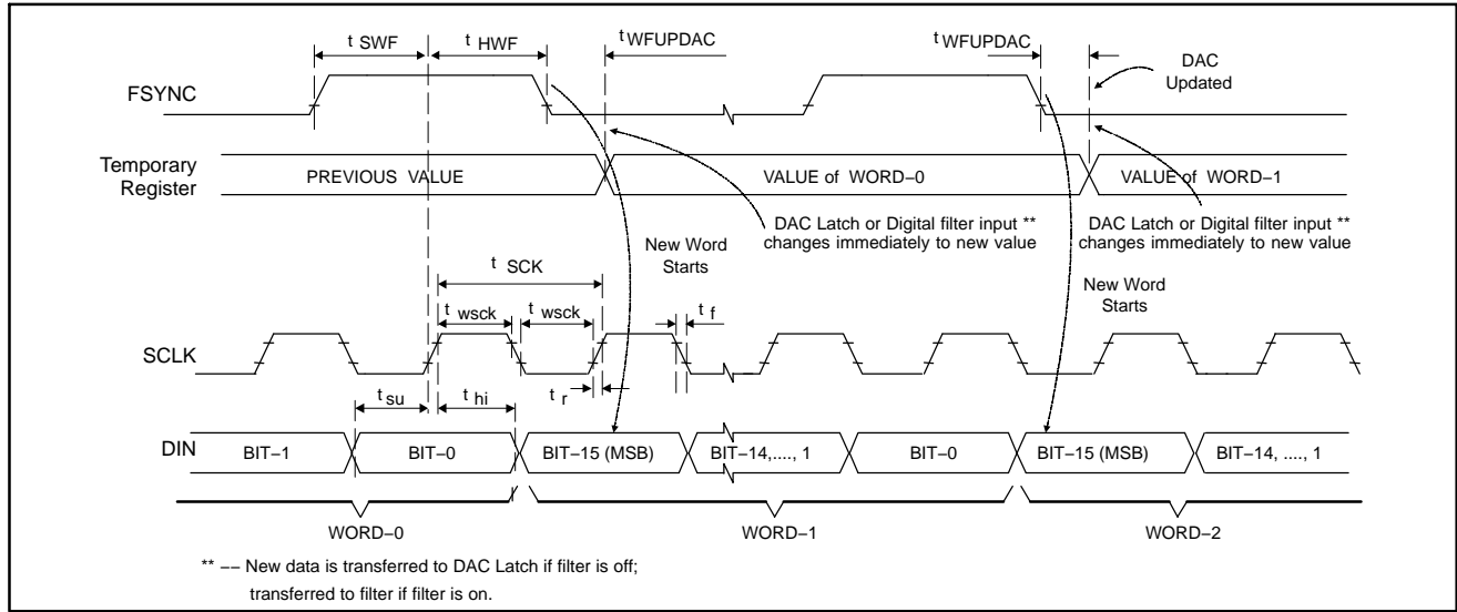
Figure 1. Timing Diagram
