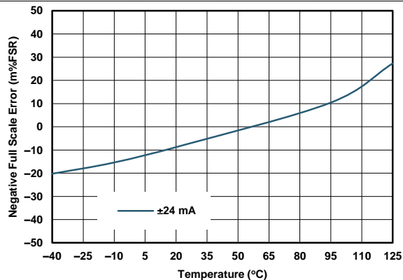
Figure 12. IOUT Full Scale Error vs Temperature
