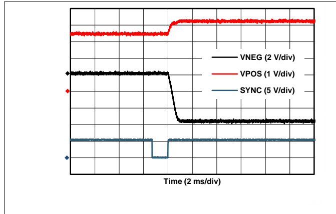
Figure 83. Buck-Boost Converter Power-On (IOUT Mode)
