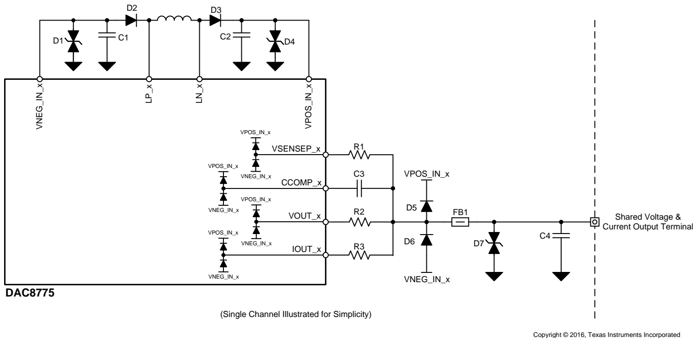
Figure 129. Simplified Block Diagram of Internal Structures and External Protection
