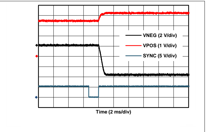
Figure 84. Buck-Boost Converter Power-On (VOUT Mode)
