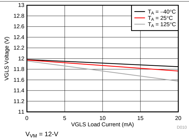
Figure 11. VGLS Voltage Over Load Current
