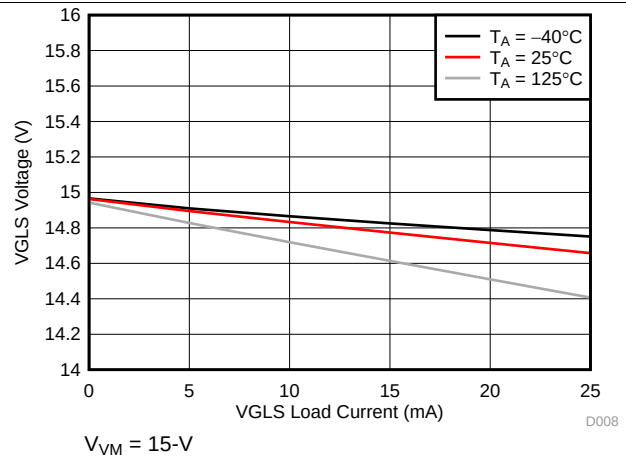
Figure 9. VGLS Voltage Over Load Current
