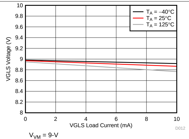
Figure 13. VGLS Voltage Over Load Current
