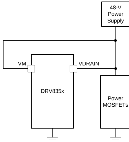
Figure 30. Single Supply Example
