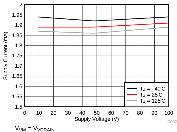
Figure 3. V DRAIN Supply Current Over Supply Voltage
