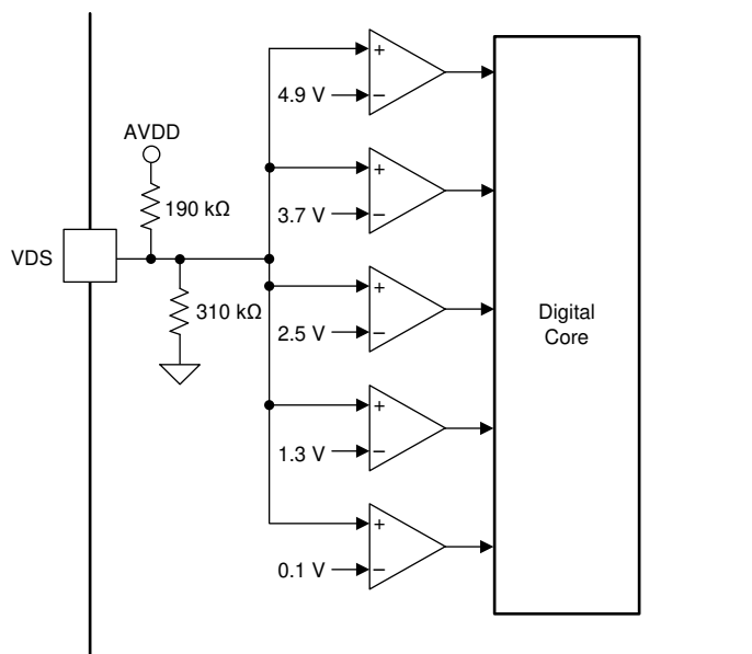
Figure 7-14. VDS Block Diagram
