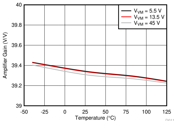
Figure 6-9. Amplifier Gain
