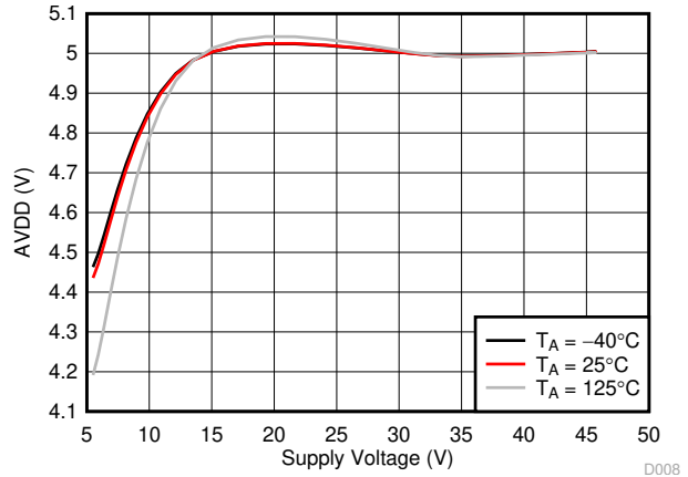
Figure 6-8. AVDD Regulator
