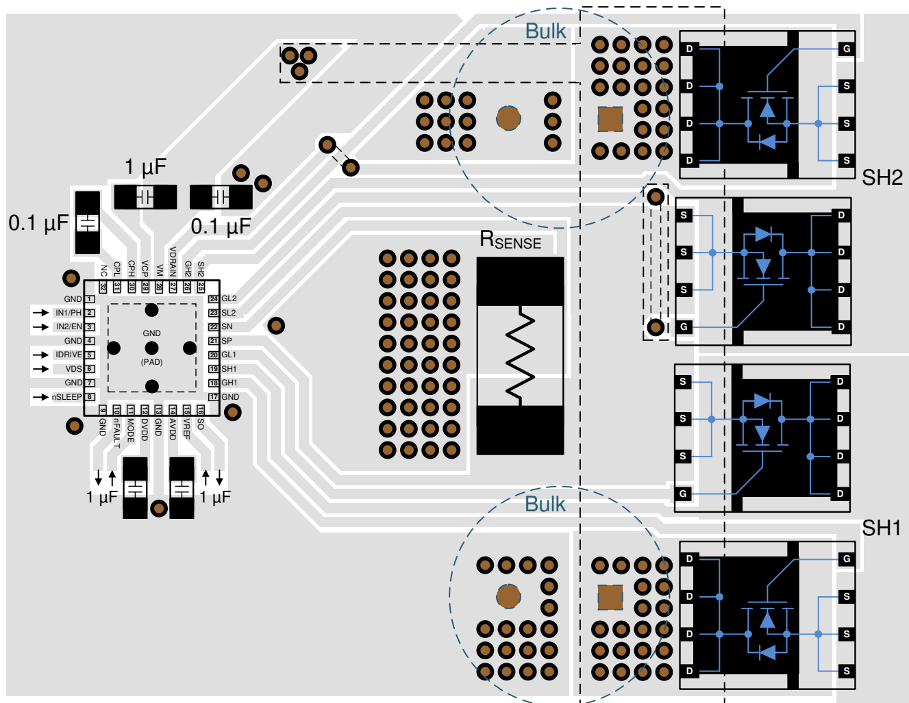
Figure 10-1. DRV8702-Q1 Layout Example
