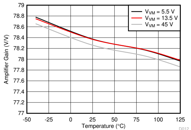
Figure 6-10. Amplifier Gain
