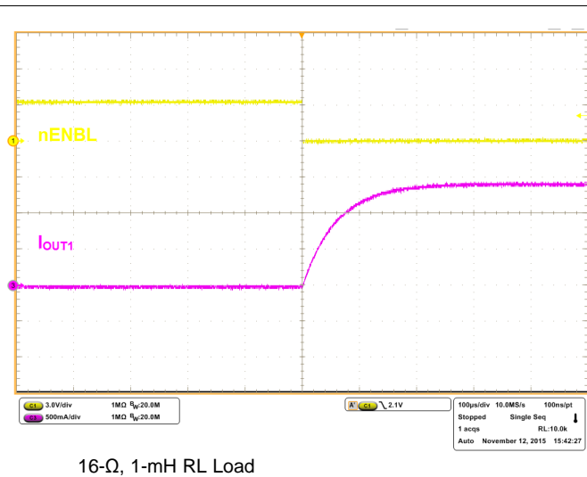
Figure 12. Current Ramp With V_M = 24\text{ V}
