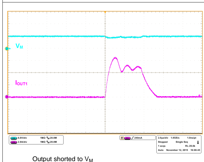
Figure 13. OCP With 8.2 V
