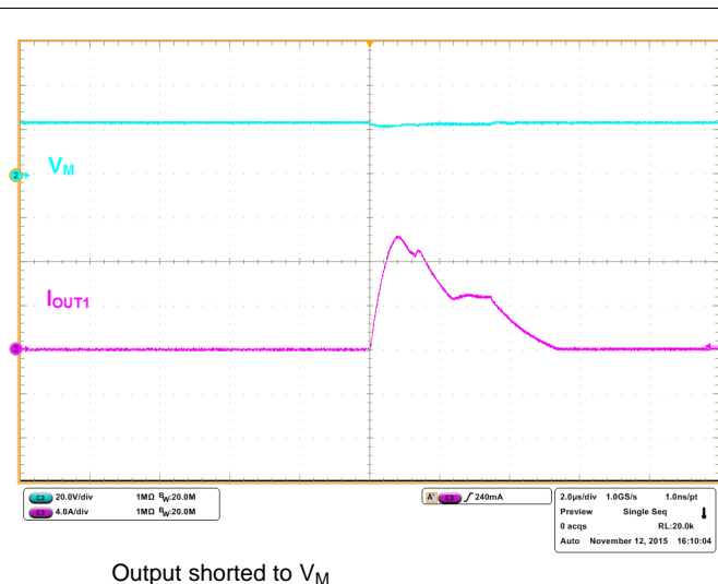
Figure 14. OCP With 24 V
