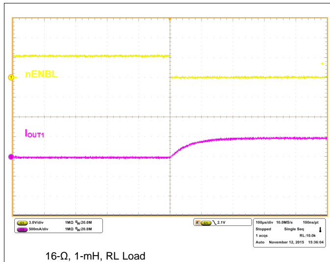
Figure 11. Current Ramp With V_M = 8.2\text{ V}
