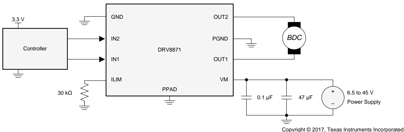
Figure 7. Typical Connections
